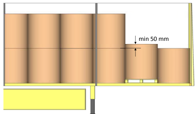
21b. Blocking of a second layer by bottom layer raised by pallets or battens
