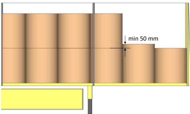
21a. Blocking of a second layer with reels of different height
