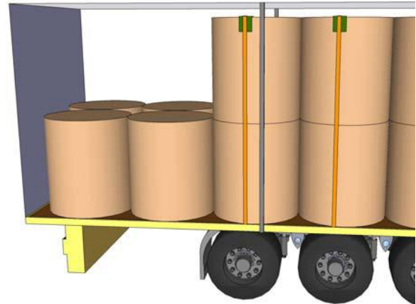
29b. Securing by top-over lashings
