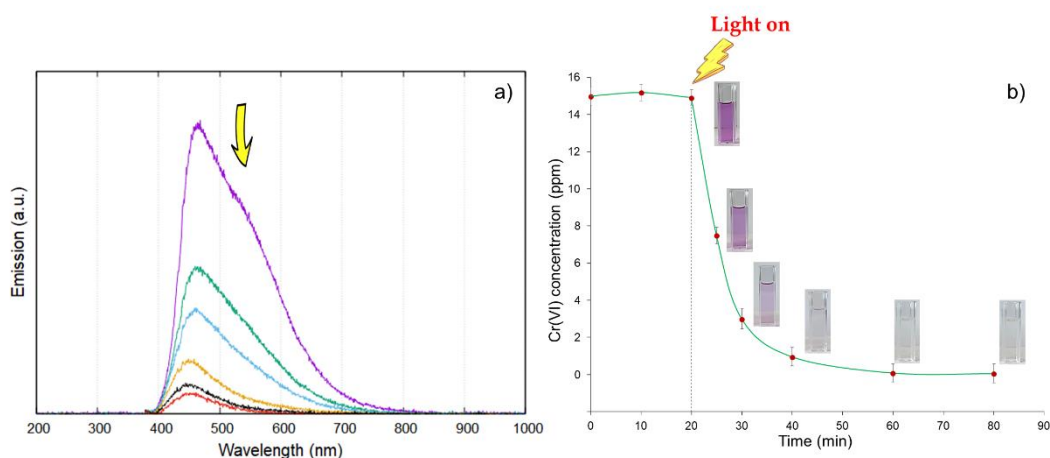
a) Decrease of pyoverdines fluorescence under UV-light radiation; b) decrease of Cr(VI) (ppm) versus time.
